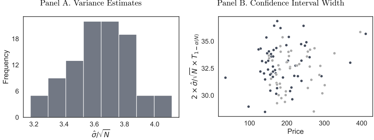
FIGURE 7: Inference Results
